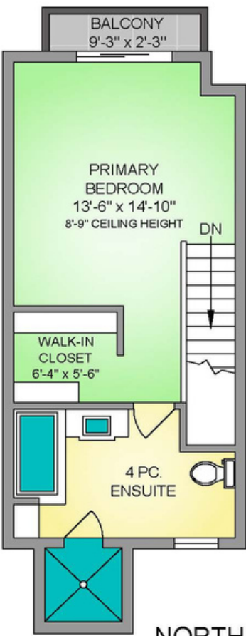
THIRD FLOOR 435 SQ. FT. 8' CEILING HEIGHT
