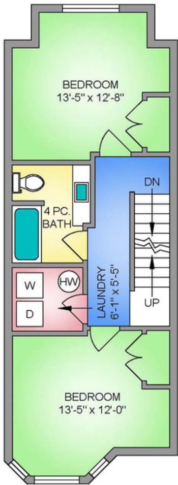
SECOND FLOOR 530 SQ. FT. 8' CEILING HEIGHT
