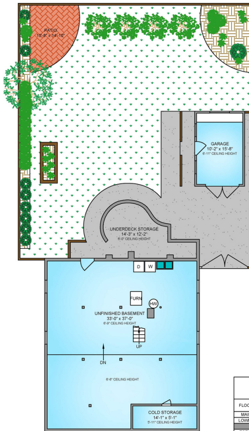
LOWER FLOOR 1218 SQ. FT. 6'-9" CEILING HEIGHT
